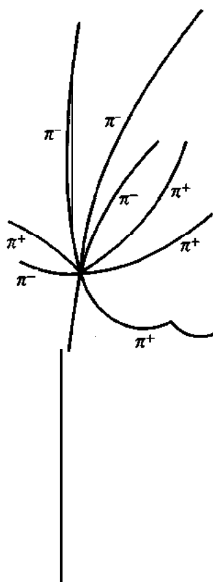
Creation of eight pions in a collision between an antiproton ( \bar{p} ) and a proton (sitting in the bubble chamber); see photograph on preceding page
