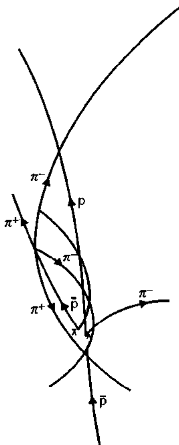
a network of reactions involving protons, antiprotons, a lambda-antilambda pair, and several pions
