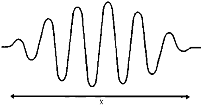
a wave packet corresponding to a particle located somewhere in the region x
