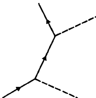
electron-photon scattering
