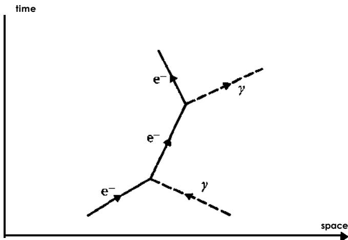
electron-photon scattering
