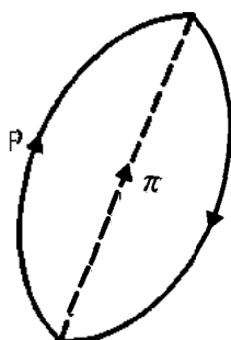
a vacuum diagram
