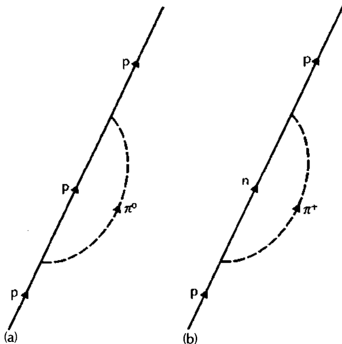
Feynman diagrams showing a proton emitting and reabsorbing virtual pions
