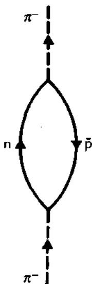
creation of a virtual neutron-antiproton pair
