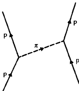
exchange of a pion ( \pi ) between two protons( p )
