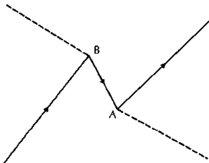
scattering process involving photons, electrons and a positron
