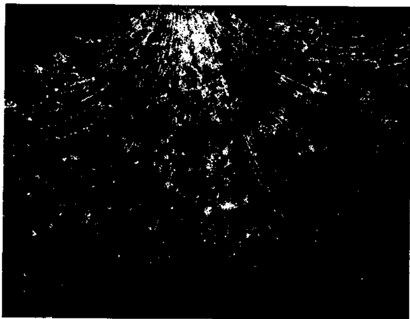
A shower of about 100 particles produced by a cosmic ray which found its way into a bubble chamber by accident. The roughly horizontal tracks in the picture belong to the particles coming out of the accelerator
