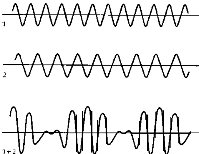
interference of two waves
