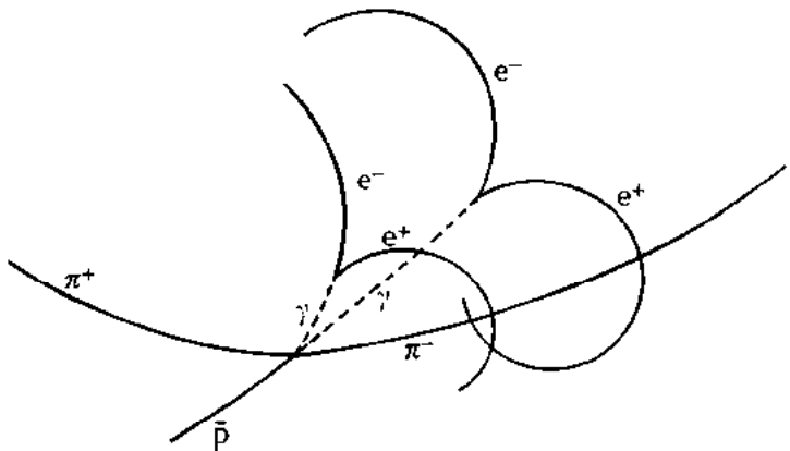
A sequence of events involving two pair creations: an antiproton ( \bar{p} ), coming from below, collides with one of the protons in the bubble chamber to create a \pi^+ (flying off to the left), a \pi^- (flying off to the right), and two photons ( \gamma ), each of which creates an electron-positron pair, the positrons ( e^+ ) curving to the right, the electrons ( e^- ) to the left.
