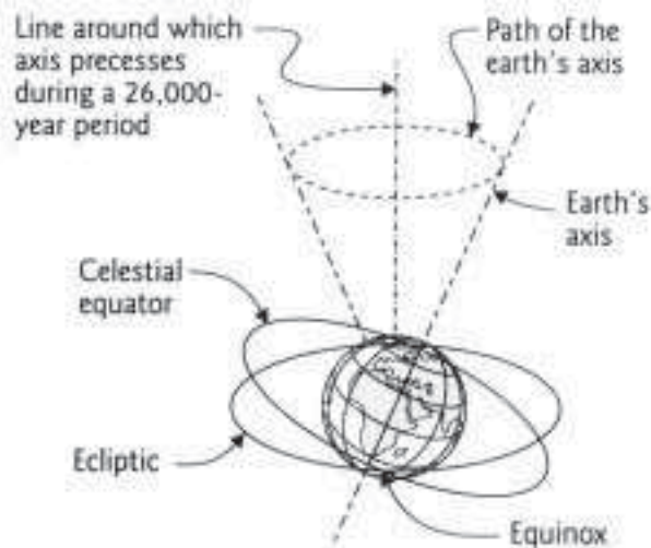
Fig. 2-39. Procession of the equinoxes (the point at which the Earth's celestial equator intersects its ecliptic) is due to the slow rotation of the Earth's axis around a perpendicular to the ecliptic.
