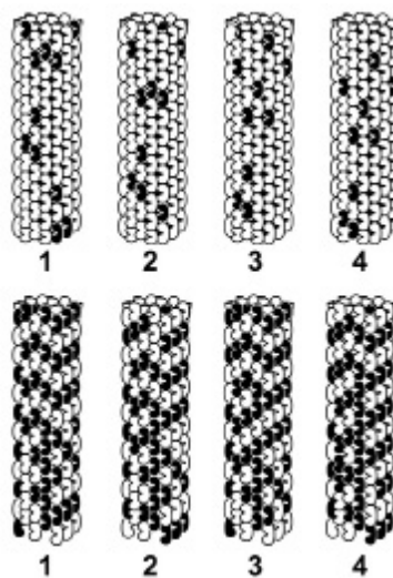
Figure 3. Microtubule automata (Rasmussen et al, 1990). Top: 4 time steps (e.g. at 8 megahertz, Pokorny et al, 2001) showing propagation of information states and patterns ('gliders' in cellular automata parlance). Bottom: At different dipole coupling parameter, bi-directional pattern movement and computation occur.
