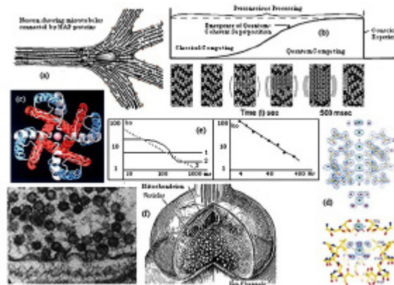
Fig 7: Features of quantum processing in proposed models. (a) Microtubule MAP proteins as envisaged in the OOR model (Hameroff and Penrose 2003). (b) The ensuing relationship between classical and quantum computing and consciousness. (c, d) gated K + ion channels from MacKinnon's group (Zhou et. al. 2001). (e) Fractal kinetics in the channels (Liebovitch et. al.) (f) Synaptic junction may invoke uncertainty of position of the vesicle.
