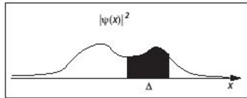
Figure 2: The probability of finding the particle within the interval \Delta is given by the black area in the figure.
