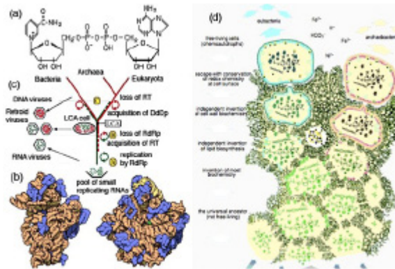
Fig 3: (a) Catalytic nicotine-adenine dinucleotide is essential in respiration. (b) Large and small subunits of the ribosome are centrally and functionally RNA [pink] (c) Molecular fossil evidence for a viral-based cellular transition from the RNA world to DNA based chromosomes, through cellular cooption of viral RNA-directed RNA-polymerase, followed by reverse transcriptase and finally DNA-dependent DNA-polymerase. (d) Independent evolution of archaean and bacterial cellular life from a non-cellular form of life at the interface of olivine and acid, iron-rich sea water forming 'lost city' undersea vents able to solve the concentration and encapsulation problems (Martin and Russell 2003).
